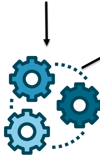
Reasoning Engine
