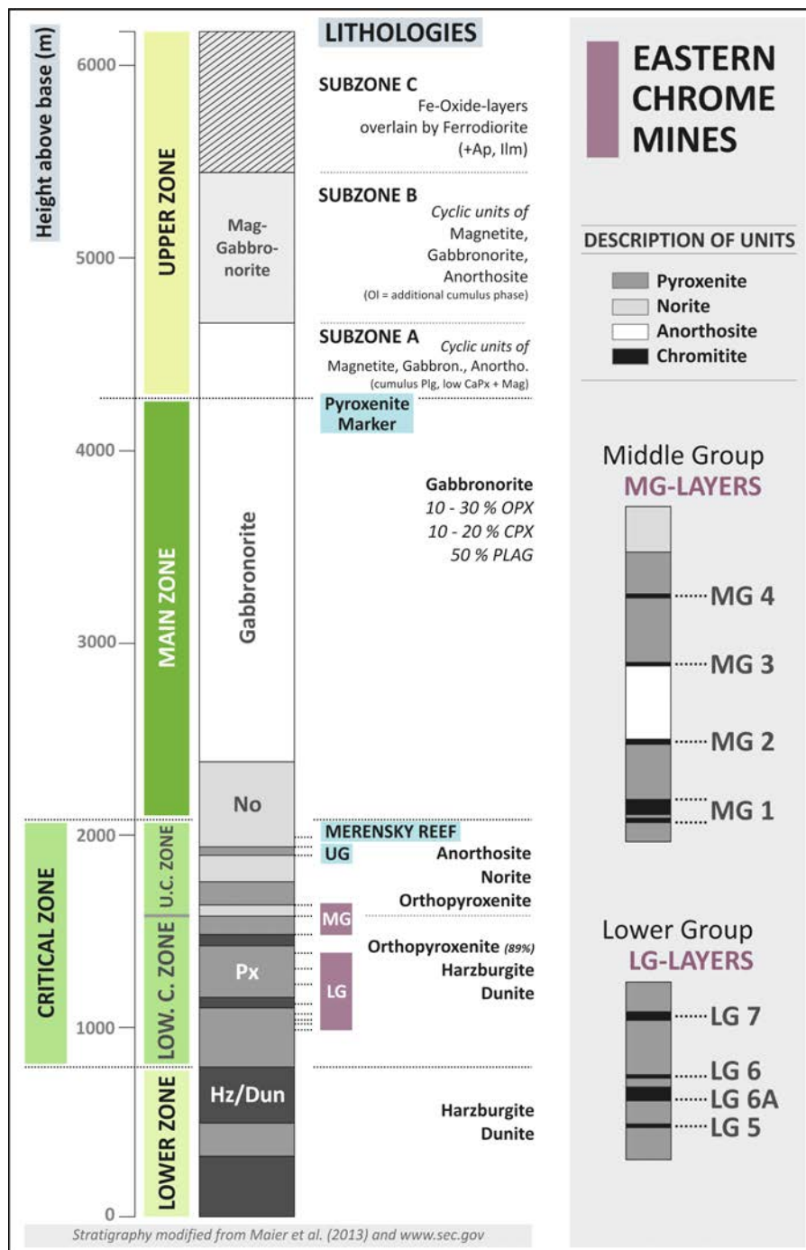
Fig. 12 Stratigraphic section of the Bushveld Complex with the Lower, Critical, Main and Upper Zones.
